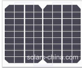
Item No: KS-M240195G 5W--18V/278mA Dimension: 240×195×5mm Tempered glass Solar Panel
