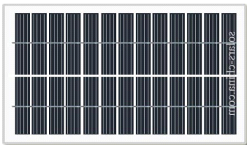
Item No. KS-M246145G 5W--13V/385mA Dimension: 246×145×5mm Tempered glass Solar Panel
