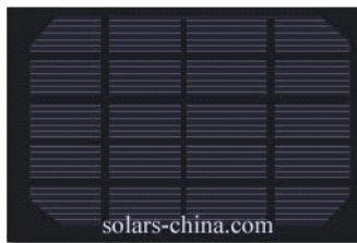
Item No: KS-M190135P 2.8W-5V/560mA Dimension:190×135×2.8mm PET Solar Panel
