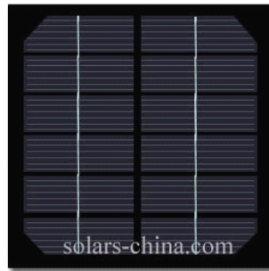
Item No: KS-M165165GB 3.6W--6V/600mA Diameter:165×165×5mm Tempered glass Solar Panel
