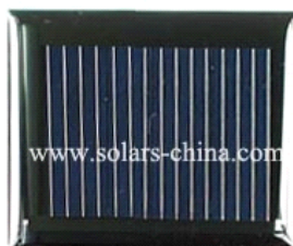
Item No. KS-M4833 4V/28mA Dimension: 48×33×3mm Epoxy Resin Solar Panel
