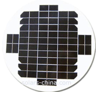
Item No: KS-Q10W 10W--18V/555mA Diameter:390mm Tempered glass Solar Panel
