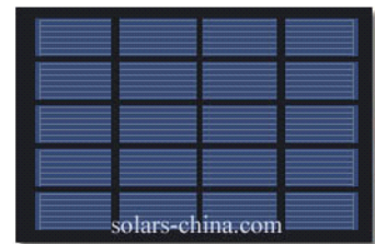
Item No: KS-P190135P 2.8W-5V/560mA Dimension:190×135×2.8mm PET Solar Panel
