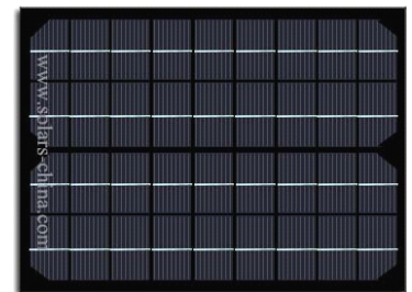
Item No: KS-M305225G 10W--18V/556mA Diameter:305×225×5mm Tempered glass Solar Panel
