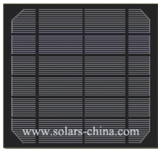
Item No. KS-M165165 3.6W--6V/600mA Dimension:165×165×2.8mm PET Solar Panel (Black)
