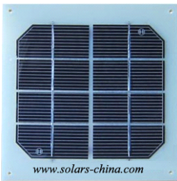
Item No: KS-M127127 1.5W-2V/750mA Dimension:190×135×2.8mm PET Solar Panel(White)
