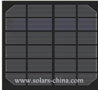
Item No: KSM175175P 3.8W-- 6V/633mA Dimension:175×175×2.8mm PET Solar Panel(Black)
