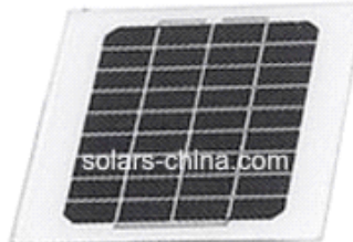
Item No: KS-M140140G 2.3W--7V/340mA Dimension: 140×140×5mm Tempered glass Solar Panel
