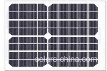
Item No. KS-M240365G 10W--18V/560mA Dimension: 240×365×5mm Tempered glass Solar Panel
