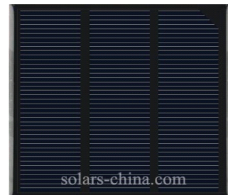
Item No. KS-M120120 1.5W -- 5V/300mA Dimension:120×120×2.8mm PET Solar Panel (Black)
